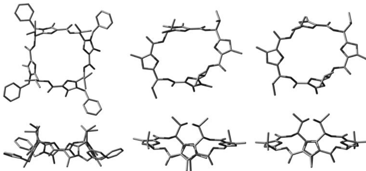
Figure 2. Molecular structures of 10 , 27 and 6 : top view (upper row) and side view (lower row); all hydrogen atoms and all solvent molecules have been omitted for clarity.
