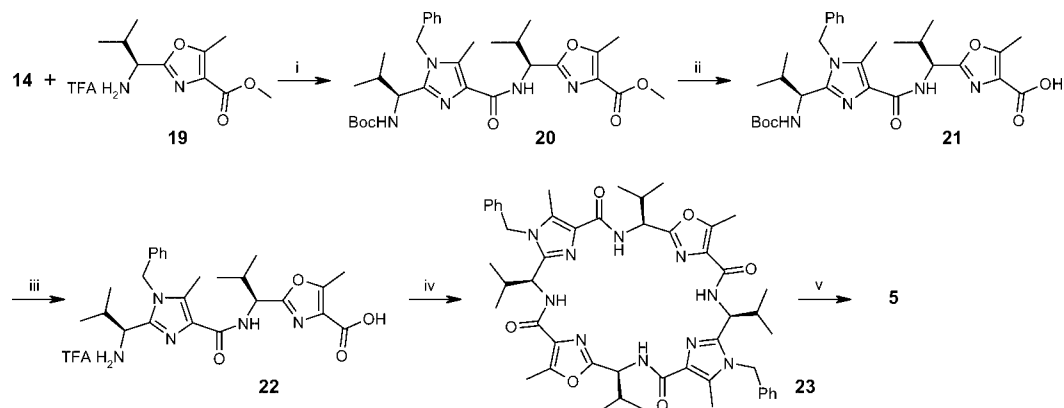
Scheme 5. Synthesis of scaffold 5 : i) FDPP, i Pr 2 NEt, CH 3 CN, room temp., 87%. ii) 2 M NaOH, MeOH/dioxane, 98%. iii) TFA, DCM, quant. iv) FDPP, i Pr 2 NEt, CH 3 CN, room temp., 55%. v) H 2 , Pd(OH) 2 , MeOH/DCM, 95%.
