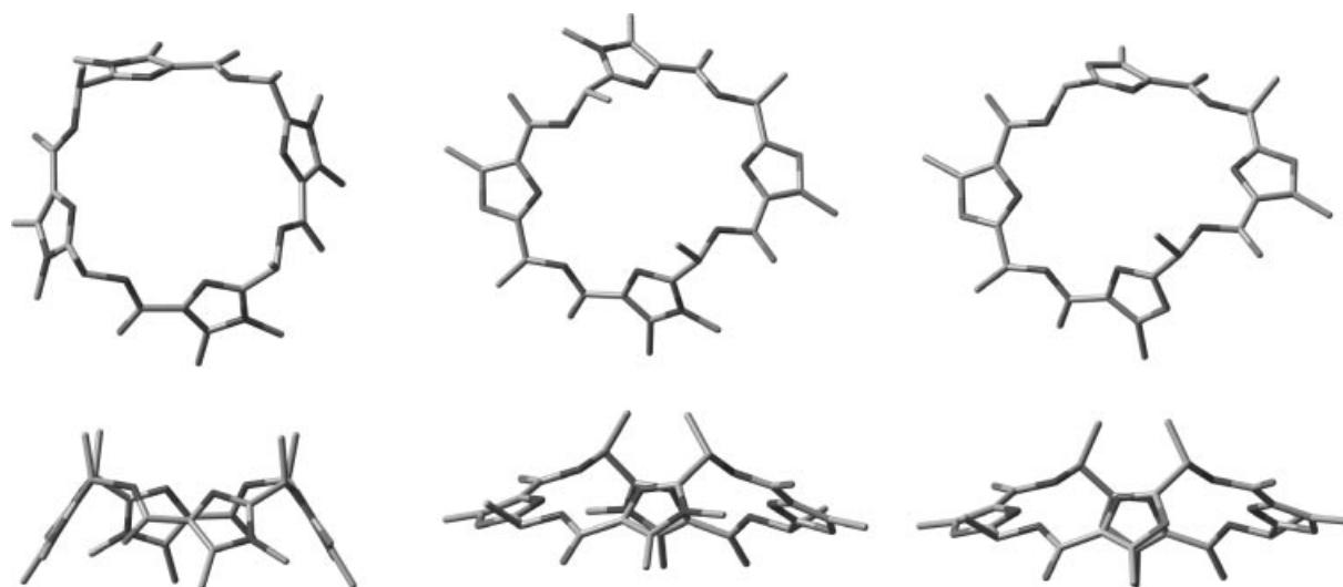
Figure 5. Molecular structures of the energetically preferred conformers of 35 (type I), 36 (type IIa) and 37 (type II) calculated with B3LYP/6-31G**: top views (upper row) and side views (lower row); all hydrogen atoms have been omitted for clarity.
