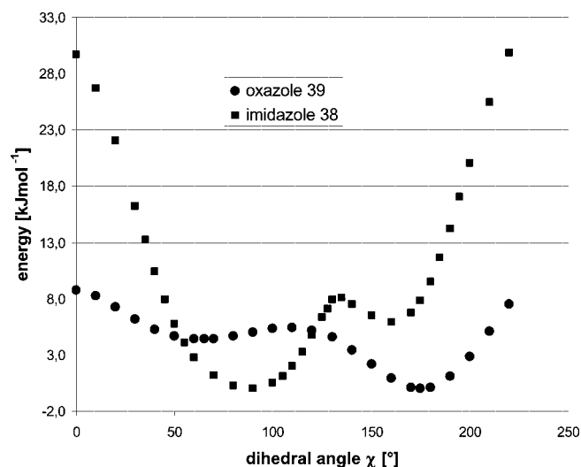
Figure 7. Calculated energy profiles in relation to the dihedral angles by use of B3LYP/6-31G**.
