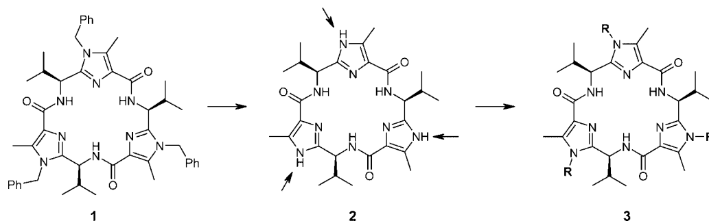
Scheme 1. Synthesis of the C_3 -symmetric molecular scaffold 2 .
