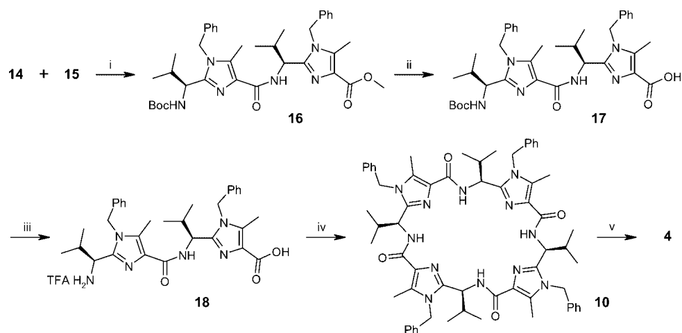
Scheme 4. Synthesis of scaffold 4 : i) FDPP, i Pr 2 NEt, CH 3 CN, room temp., 78%. ii) 2 M NaOH, MeOH/dioxane, 95%. iii) TFA, DCM, quant. iv) FDPP, i Pr 2 NEt, CH 3 CN, room temp., 65%. v) H 2 , Pd(OH) 2 , MeOH/DCM, 97%.
