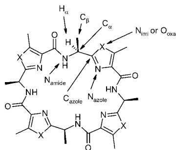
Figure 3. Definition of the abbreviations used.
