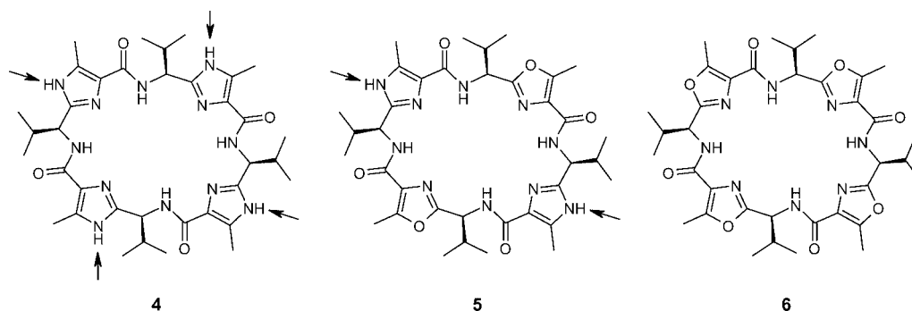
Figure 1. Structures of C_4 - and C_2 -symmetric molecular scaffolds.
