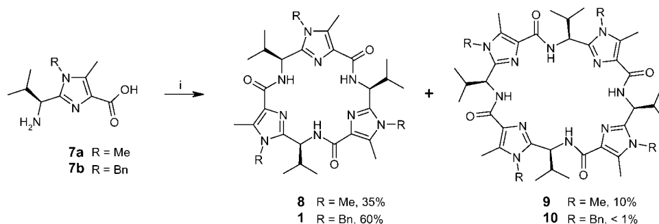
Scheme 2. i) FDPP, iPr_2NEt , CH_3CN , room temp.
