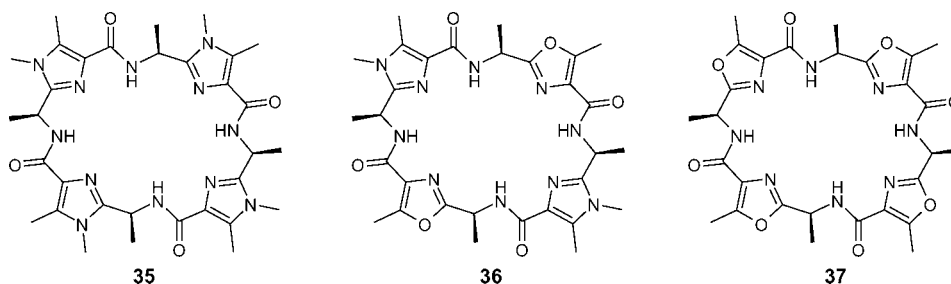
Figure 4. Structures of the cyclic peptides investigated by gas-phase calculations.
