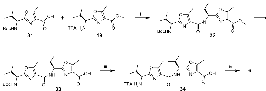
Scheme 8. Synthesis of cyclopeptide 6 . i) FDPP, i Pr 2 NEt, CH 3 CN, room temp., 74%. ii) 2 M NaOH, MeOH/dioxane, 95%. iii) TFA, DCM, quant. iv) FDPP, i Pr 2 NEt, CH 3 CN, room temp., 72%.
